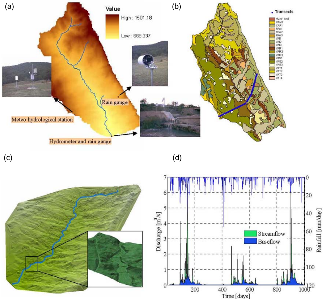
Fig. 2 Characteristics of the Fiumarella di Corleto catchment: digital elevation model ( 1 \times 1 m) and instrumentation (a), land system (b), 3-D elaboration morphology (c) and basin response with the definition of the superficial runoff and base flow components obtained using a mathematical filter (see Manfreda et al. , 2003) (d).
